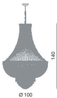
Washington sospensione Ø 100 cm Ø 100 cm - H 140 cm 18 x E14 40W
