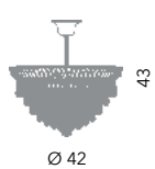
Naples sospensione Ø 40 cm Ø 42 cm - H 43 cm 4 x E14 40W
