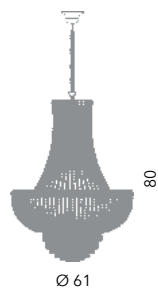
Washington sospensione Ø 60 cm Ø 61 cm - H 80 cm 9 x E14 40W
